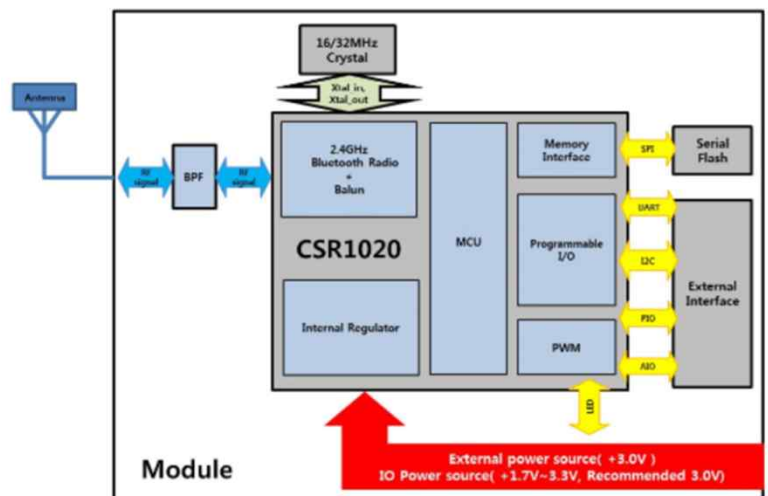
MD-CLESN20 Block Diagram
