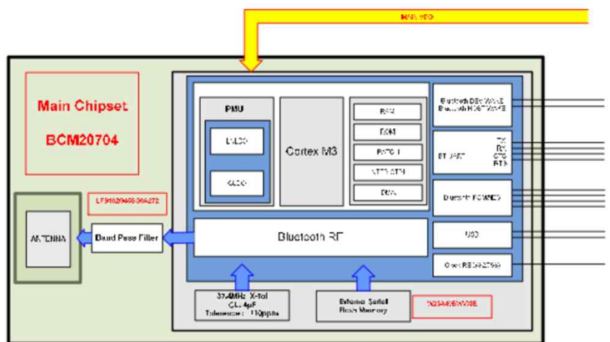
MD-BC100 Block Diagram
