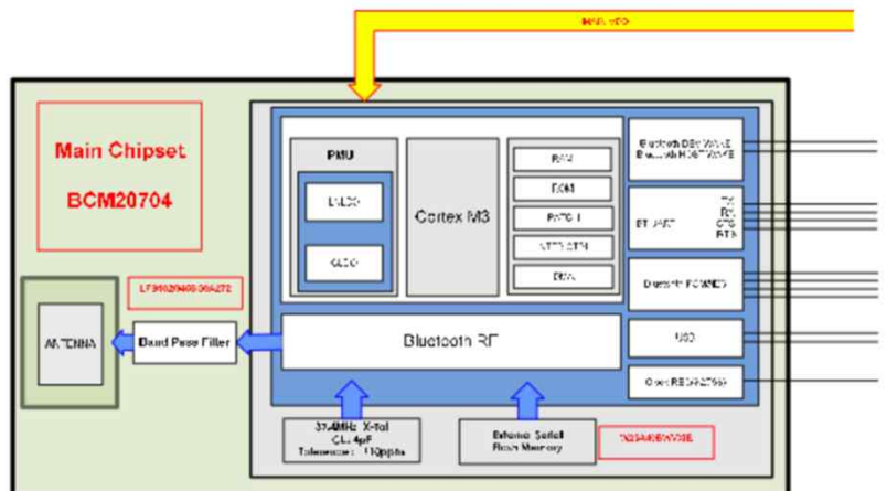
MD-8RFH Block Diagram
