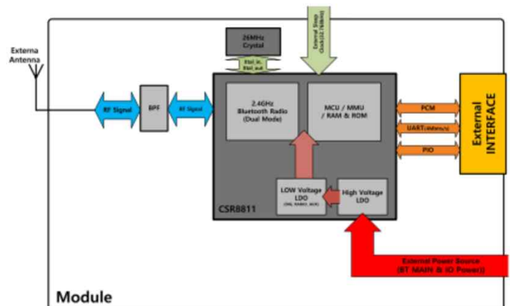
MD-8RFS Block Diagram
