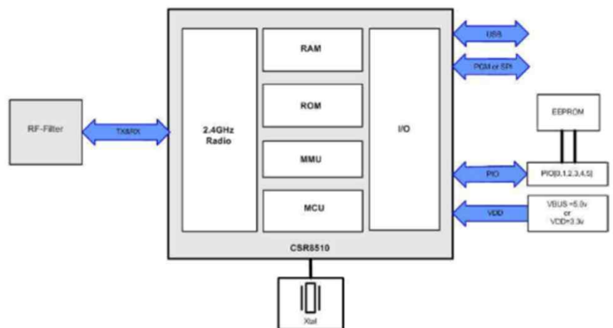
MD-8RFH Block Diagram
