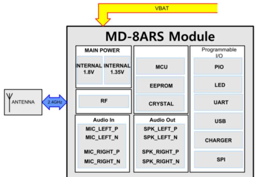
MD-8ARS Block Diagram
