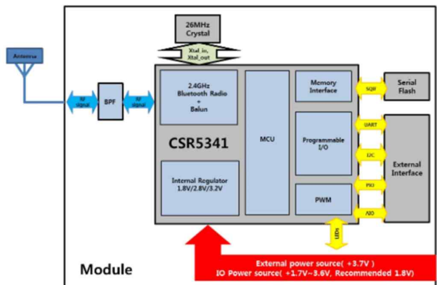
MD-5DRB41 Block Diagram
